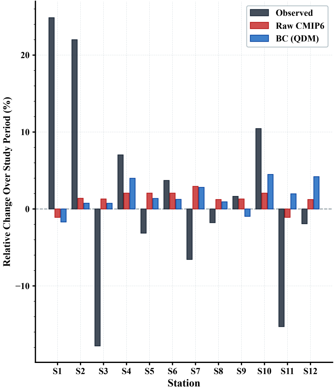
(c) Relative Rainfall Change = (Slope × N_years) / Mean × 100%
