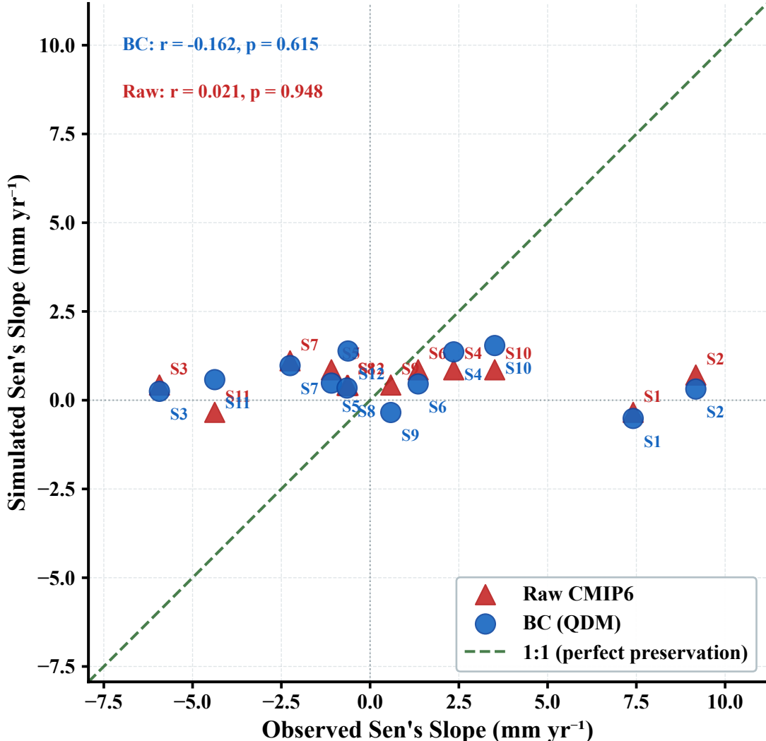
(b) Trend Preservation Assessment Simulated vs Observed Sen's Slope Closer to 1:1 line = better preservation
