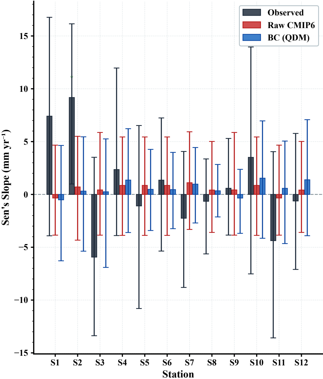
(a) Sen's Slope per Station Bars = 95% CI | *** p < 0.001 ** p < 0.01 * p < 0.05
